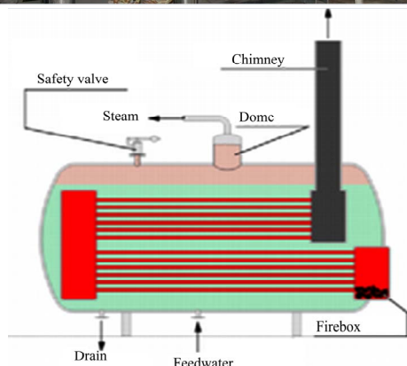
Figure 6. Fire-tube boiler.
